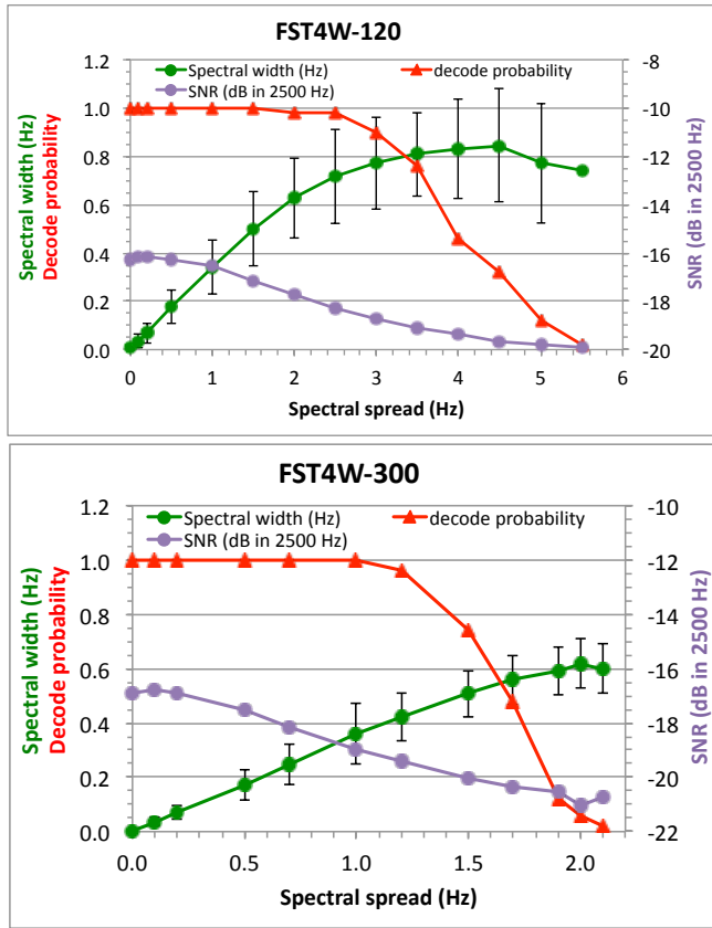
Figure 5. Variation of spectral width, decode probability and SNR with spectral spread from 50 runs of the fst4sim model at each value of Doppler spread for -120 upper, and -300 lower. The bars on spectral width are at \pm 2.5 times the standard deviation, that is, 99% of the values lie within the interval.
