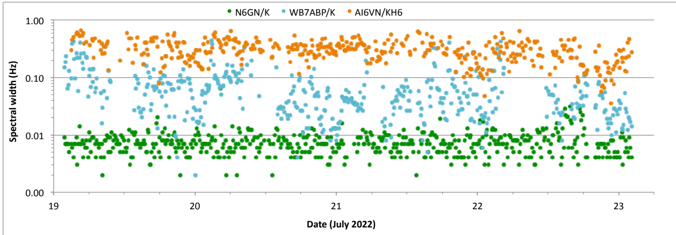
Figure 9. Time series of the spectral width on a log scale as output by jt9 from FST4W-300 transmissions by N6GN for three different propagation paths to: (green) N6GN/K a KiwiSDR with GPSDO at 21 km; (cyan) WB7ABP/K a KiwiSDR with GPSDO at 1558 km; (orange) AI6VN/KH6 a KiwiSDR with standard GPS aiding at 5291 km.
