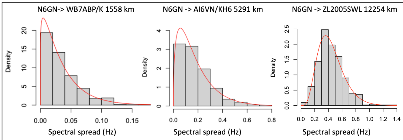
Figure 10. Histograms of spectral spread for the ionospheric path only, derived using the method in the Annex, for three paths from N6GN, Fort Collins, Co., to WB7ABP/K, Santa Rosa, Ca., AI6VN/KH6, Maui, Hi., and ZL2005SWL, North Island, New Zealand. To WB7ABP/K and AI6VN/KH6 transmissions were FST4W-300, and FST4W-120 to ZL2005SWL.
