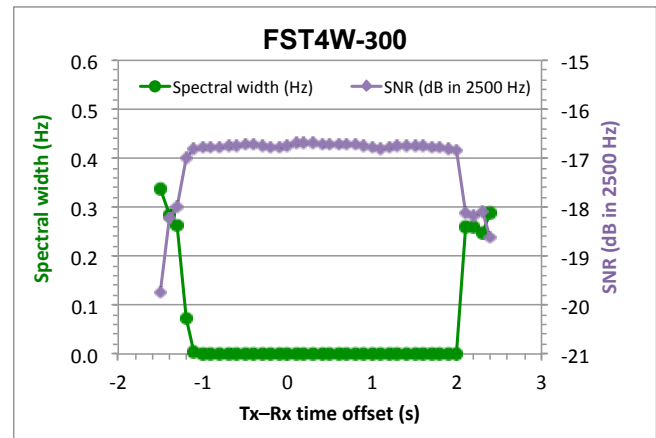
Figure 4. Variation of SNR and spectral with from fst4sim with time offset between transmitter and receiver for -300, showing biased values at each extreme but before no decode is possible.
