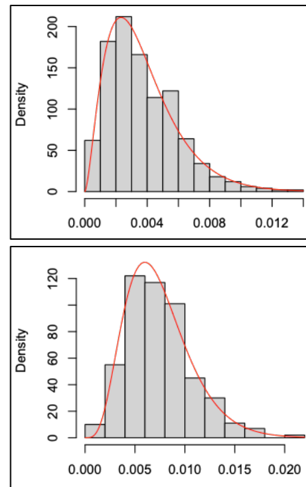
Figure A2. (upper) Histogram with fitted Gamma distribution for the N6GN/K GPSDO receiver only, formed by halving the Shape parameter from Figure A1 keeping the same Scale. (lower) Synthesised distribution for the transmitter and receiver to compare with Figure A1 (lower).
