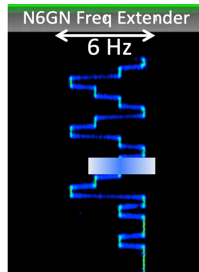
Figure 3. Waterfall display of the spectrum of the 33rd harmonic of a 14 MHz local FST4W-120 transmission from on ANAN SDR at N6GN using a KiwiSDR with GPSDO and a homebrew frequency extender. The image shows the smooth transitions between tones and the fraction of a tone period they span. The rectangle at the centre represents additional spectral spreading.
