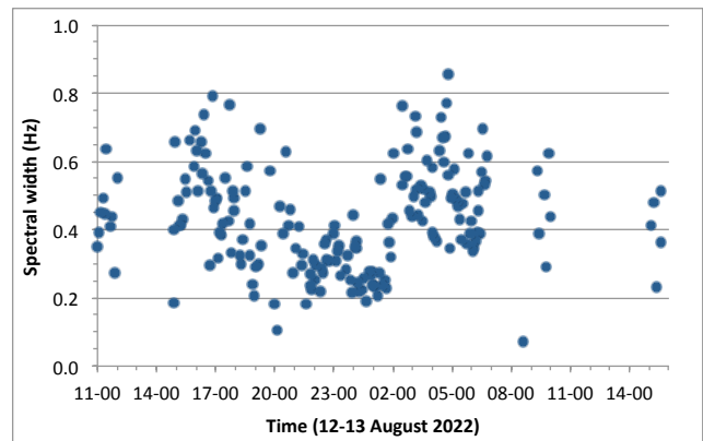
Figure 12. Time series of the spectral width of FST4W-120 transmissions from K6PZB received at KFS using its SW antenna. The separation is 124 km - why the large spectral widths? They were much greater than those from N6GN at 1535 km via the ionosphere at this time.
