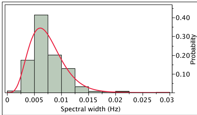
Figure 6. Histogram of the distribution of FST4W-300 spectral width determinations with GPSDO transmitter N6GN and GPSDO receiver N6GN/K over a 21 km line of sight path, from 543 spots 19-23 July 2022. In red is a fitted Gamma distribution, shape=5.62 and scale=0.00132.
