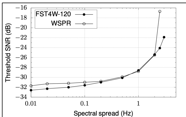
Figure 1. A comparison of the decode threshold with spectral spread for WSPR and FST4W-120. Acknowledgement: Based on figure provided by Steve Franke K9AN.
