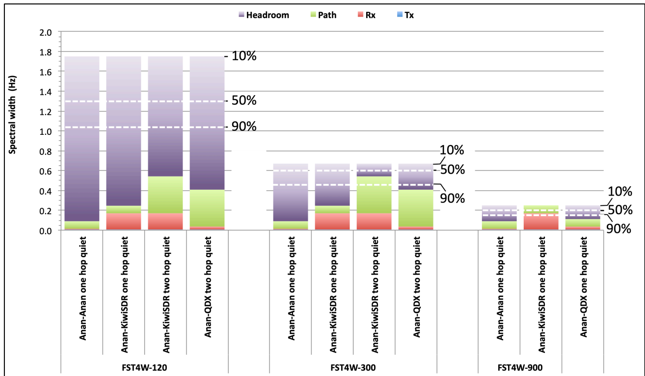
Figure 8. Spectral spread budgets for FST4W-120 to -900 for example combinations of transmitter, receiver and ionospheric propagation on the 20 m band. The upper limit for each column is the spectral spread at which there is only a 10% probability of decoding the signal. Also marked are the limits for 50% and 90% decode probability. While these lines remain in the purple 'headroom' area decode should be possible for quiet conditions ( K_p < 3 ).
