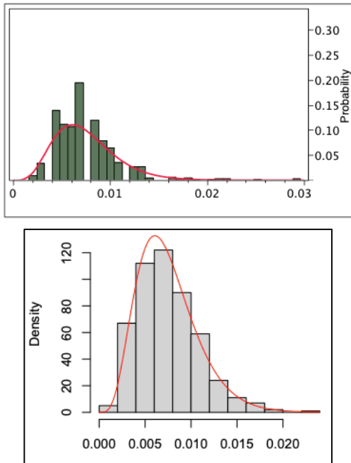
Figure A1. (upper) Histogram of actual spectral width values in Hz over a 21 km line-of-sight path from N6GN to N6GN/K with identical GPSDO master oscillators at the transmitter and receiver with a best-fit Gamma distribution. (lower) A synthesised histogram of a Gamma distribution of 500 values with the same Scale and Shape parameters as the observations.
