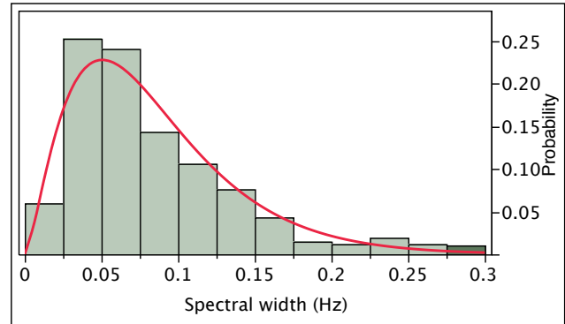
Figure 7. Two measures of short-term frequency variation in two KiwiSDRs. Upper: Histogram and fitted Gaussian distribution at G3ZIL of frequency error at 10 MHz at one-second intervals. Lower: Spectral width from jt9 at KPH from FST4W-120 GPSDO transmissions from K6PZB over a 38 km path.
