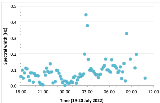
Figure 11. Time series of the spectral width of FST4W-300 transmissions from N6GN received at WB7ABP/K with suggestion of periodic variations, times with very low scatter, an event around 03:00 UTC and a slow rise toward the band closing.
