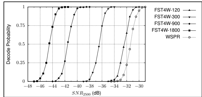
Figure 2. How decode probability varies with SNR near the threshold for FST4W-120 to -1800 in comparison with WSPR. Acknowledgement: figure provided by Steve Franke K9AN.
