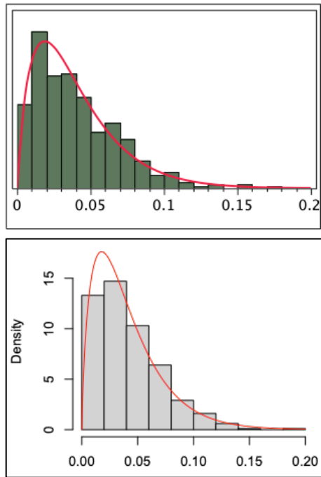
Figure A3. (upper) Histogram with fitted Gamma distribution for the total path from N6GN to WB7ABP/K including contributions from the transmitter and receiver. (lower) Synthesised distribution for the total path to compare with Figure A3 (upper).
